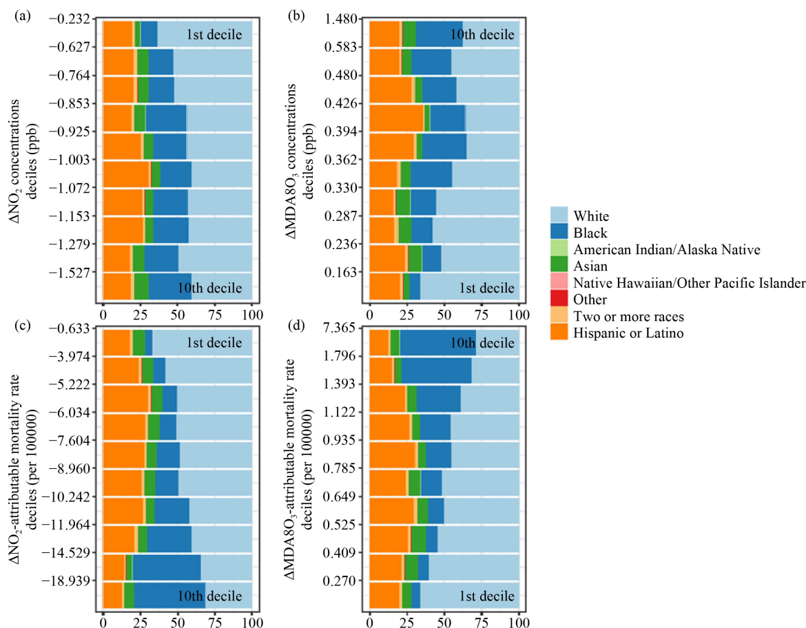
Fig. 6 Deciles of (a, b) change in \text{NO}_2 and MDA8 \text{O}_3 concentrations between an ACT policy scenario and baseline and (c, d) change in \text{NO}_2 and MDA8 \text{O}_3 attributable mortality rates stratified by race and ethnic composition over the Greater Chicago region.
