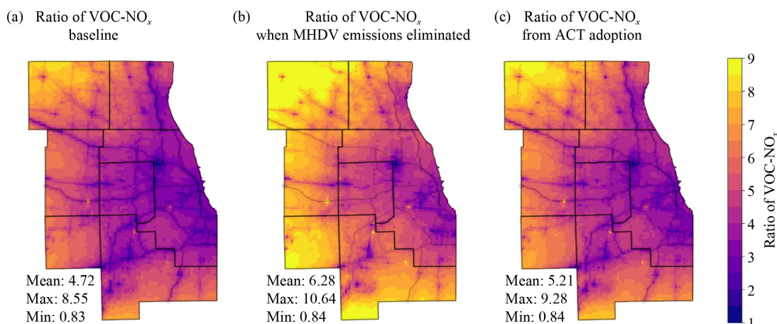
Fig. 5 WRF-CMAQ simulated annualized mean (August and October 2018, January and April 2019) volatile organic compounds (VOC) to NO x ratios for (a) baseline, (b) 100% zero-emission MHDV scenario and, (c) an Illinois Advance Clean Trucks policy scenario over the Greater Chicago region (Cook, DuPage, Kane, Kendall, Lake, McHenry, and Will Counties).
