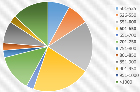
Magnitude of Chloride Exceedances in the Lower Des Plaines River Watershed, 2003 - 2018 (Ranges in mg/L)
