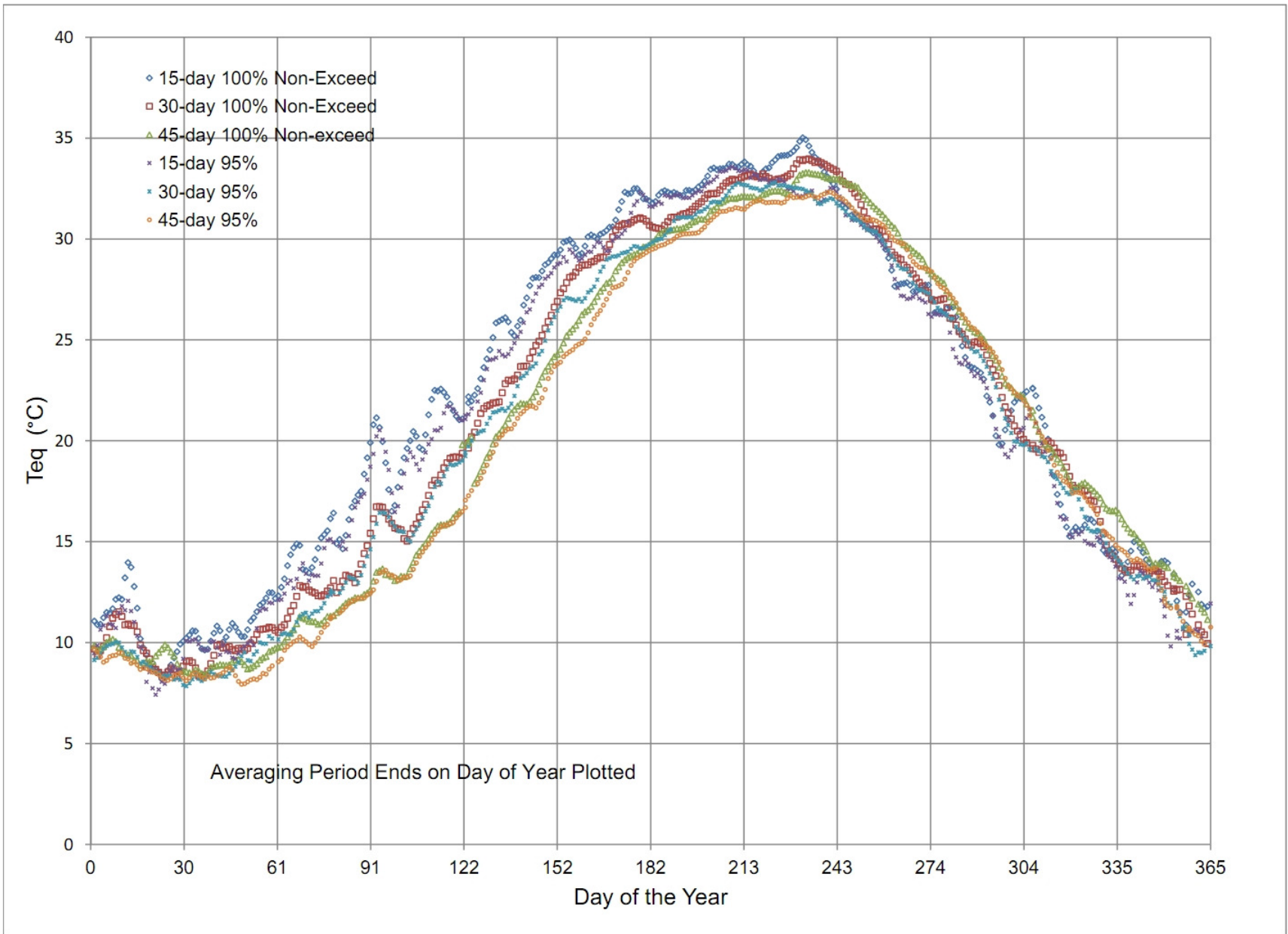
Figure F-1. Calculated Daily T_{eq} Percentile Values (15-, 30- and 45-Day Average) (SIU Climate Station Period of Record)
