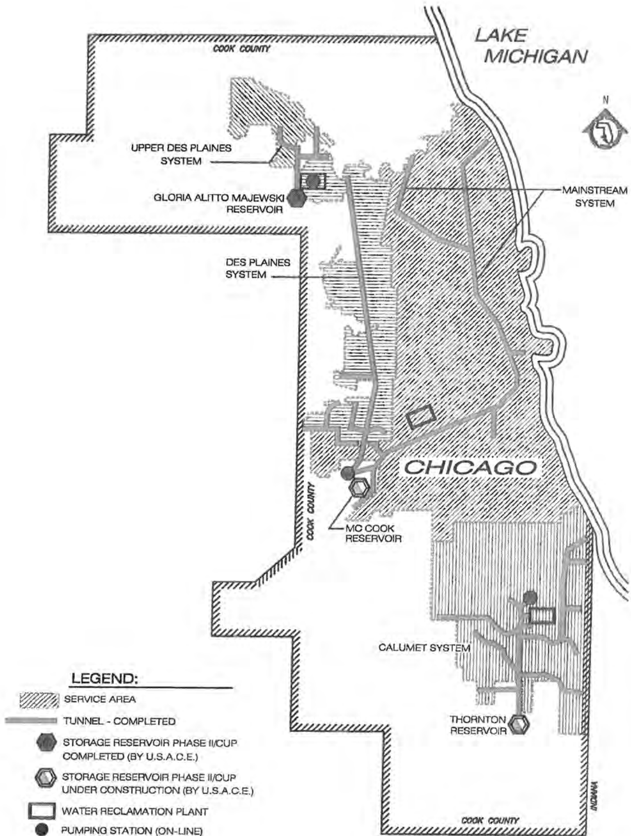
Figure 3: Tunnel and Reservoir Plan Project Status
