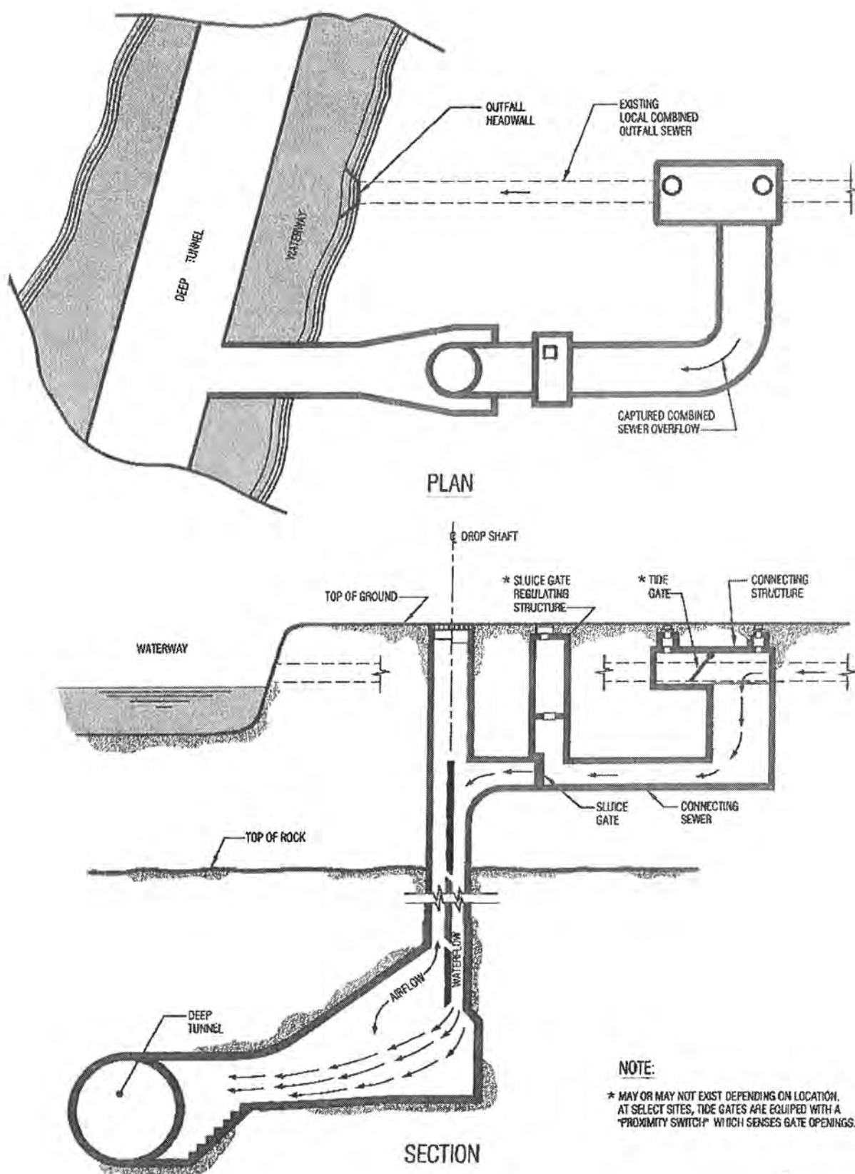
Figure 4: Drop Shaft Schematic
